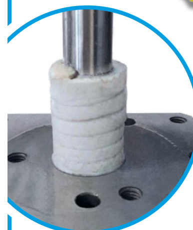
Teflon Seal for gear pump
