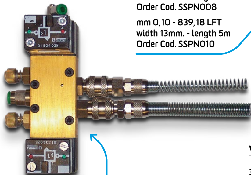
Adhesive head piston movimentation
