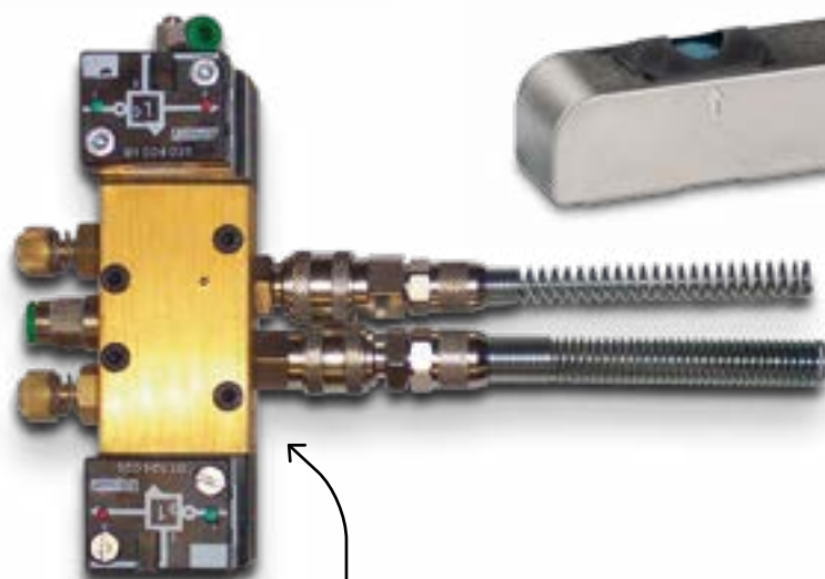
Adhesive head piston movimentation Order Cod. MA138.10.00
